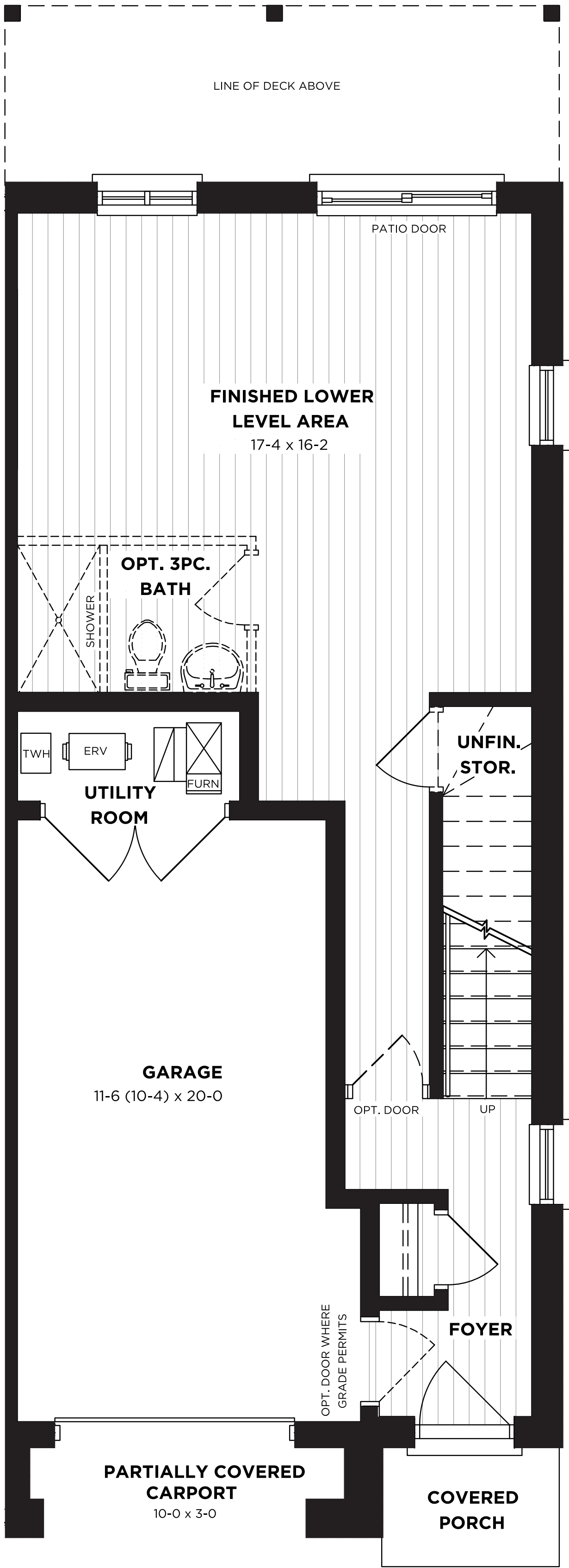
GROUND FLOOR
