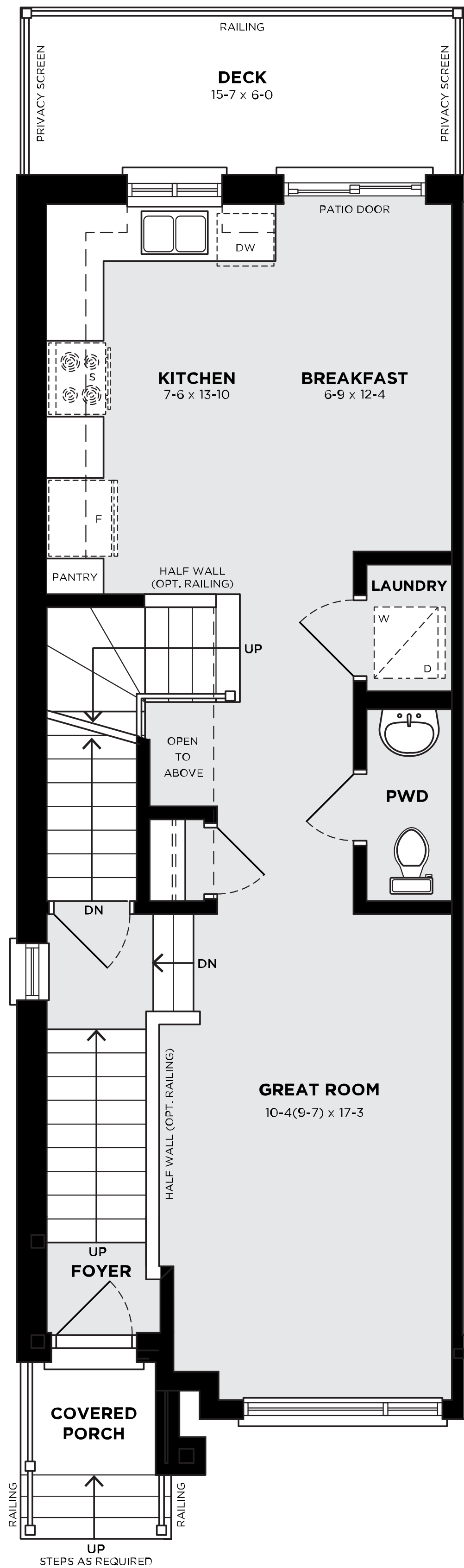
MAIN FLOOR
