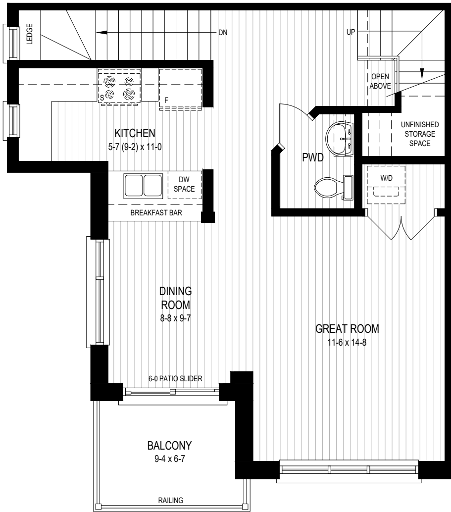
MAIN FLOOR
