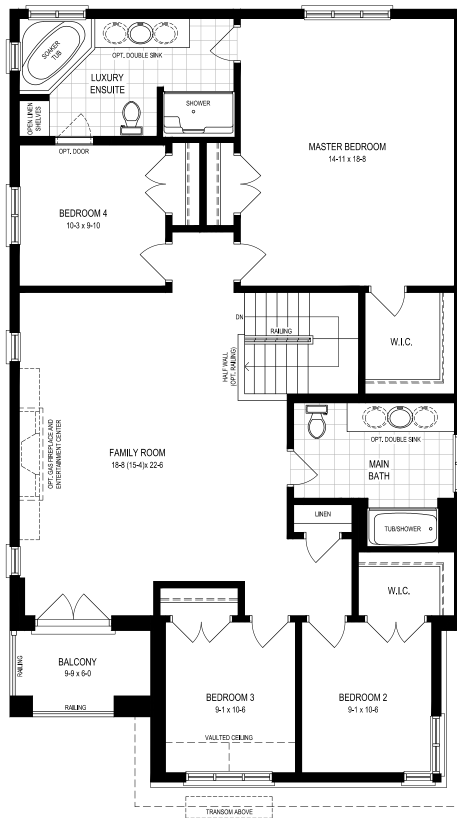
CHATEAU - S1, SECOND FLOOR
