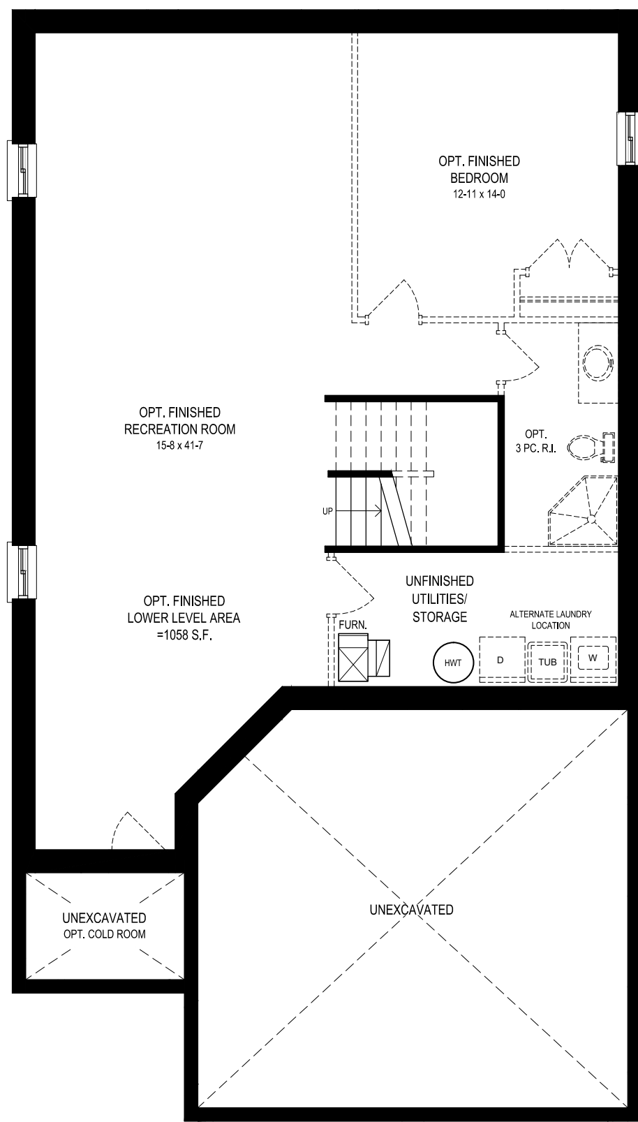
CHATEAU - B1, LOWER LEVEL
