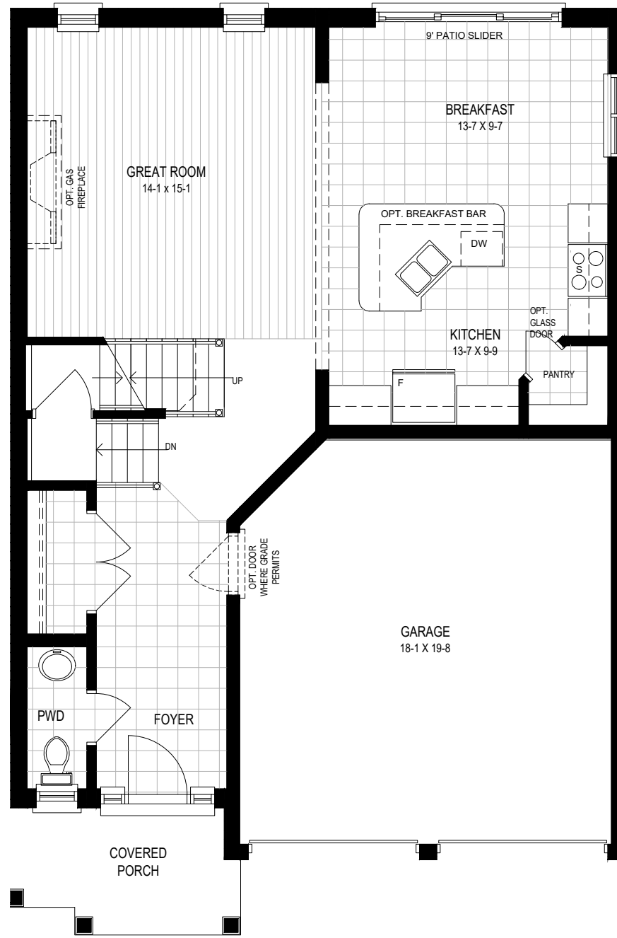
M1, MAIN FLOOR
