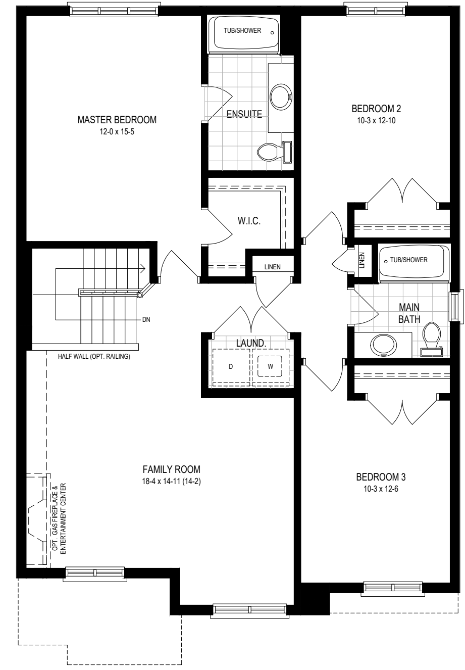
S1, SECOND FLOOR
