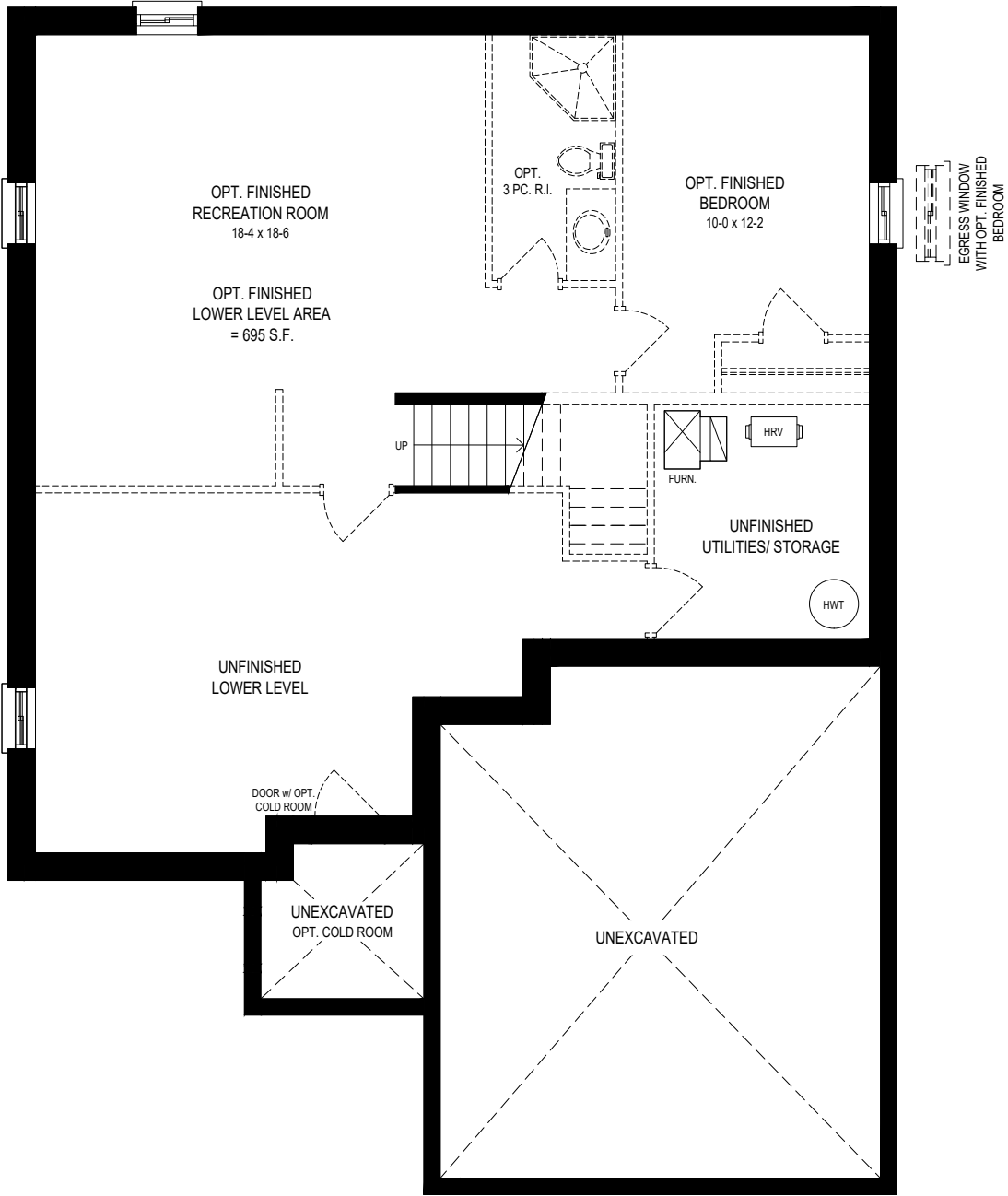
B1, LOWER LEVEL
