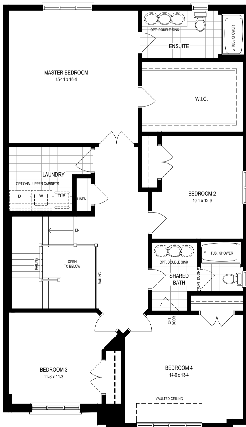
CHÂTEAU - S1, SECOND FLOOR
