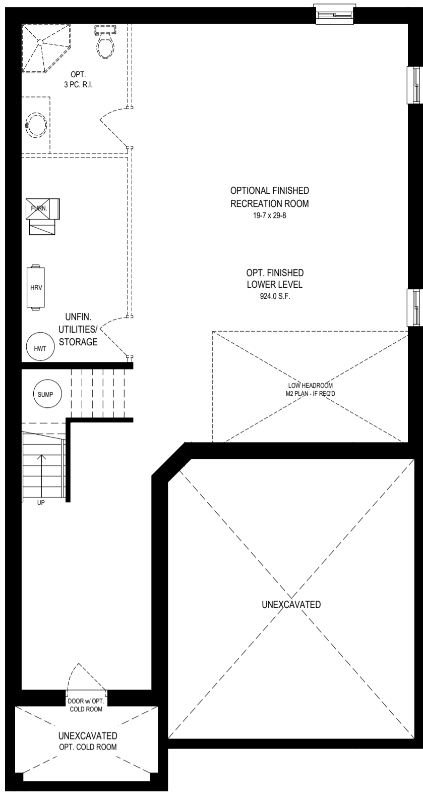
ALL ELEVATIONS - B1, LOWER LEVEL
