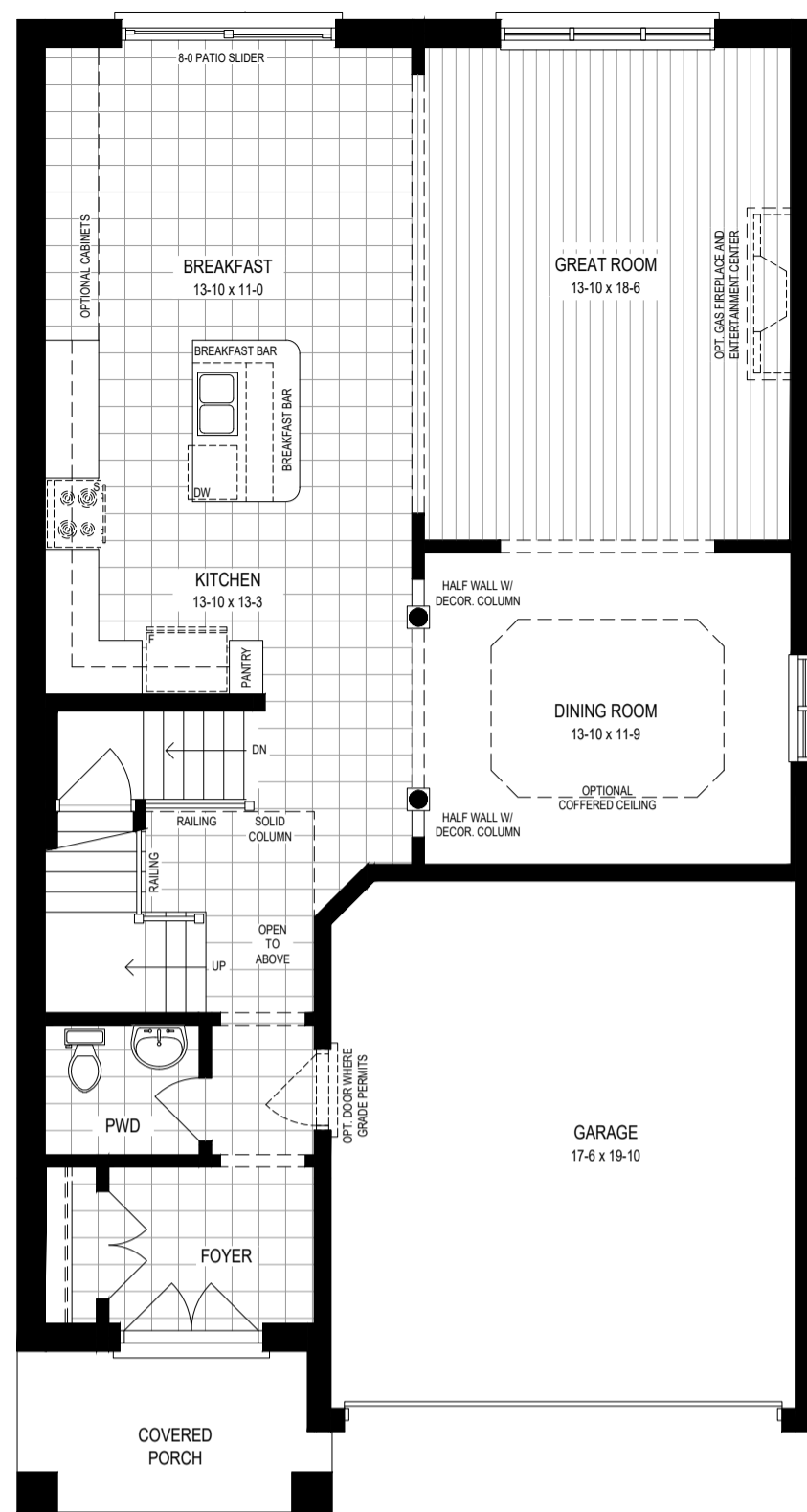
CHÂTEAU, TRADITIONAL & MODERN - M1, MAIN FLOOR
