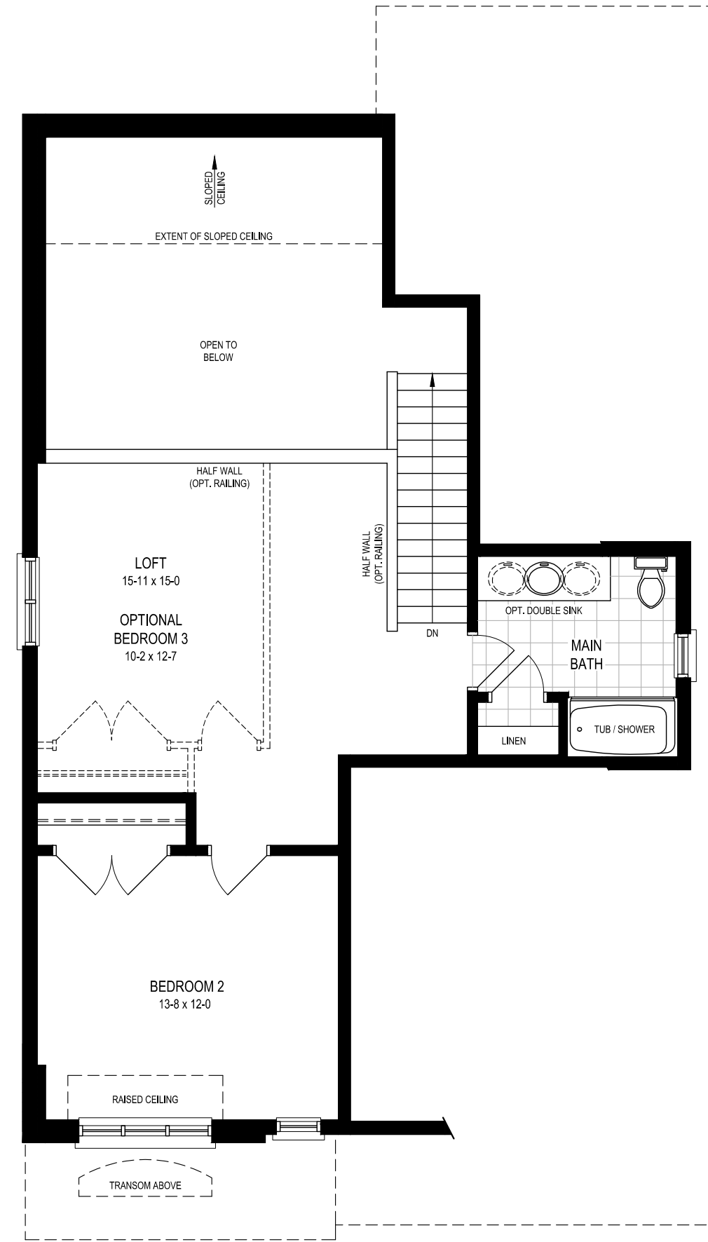
CHÂTEAU - S1, SECOND FLOOR
