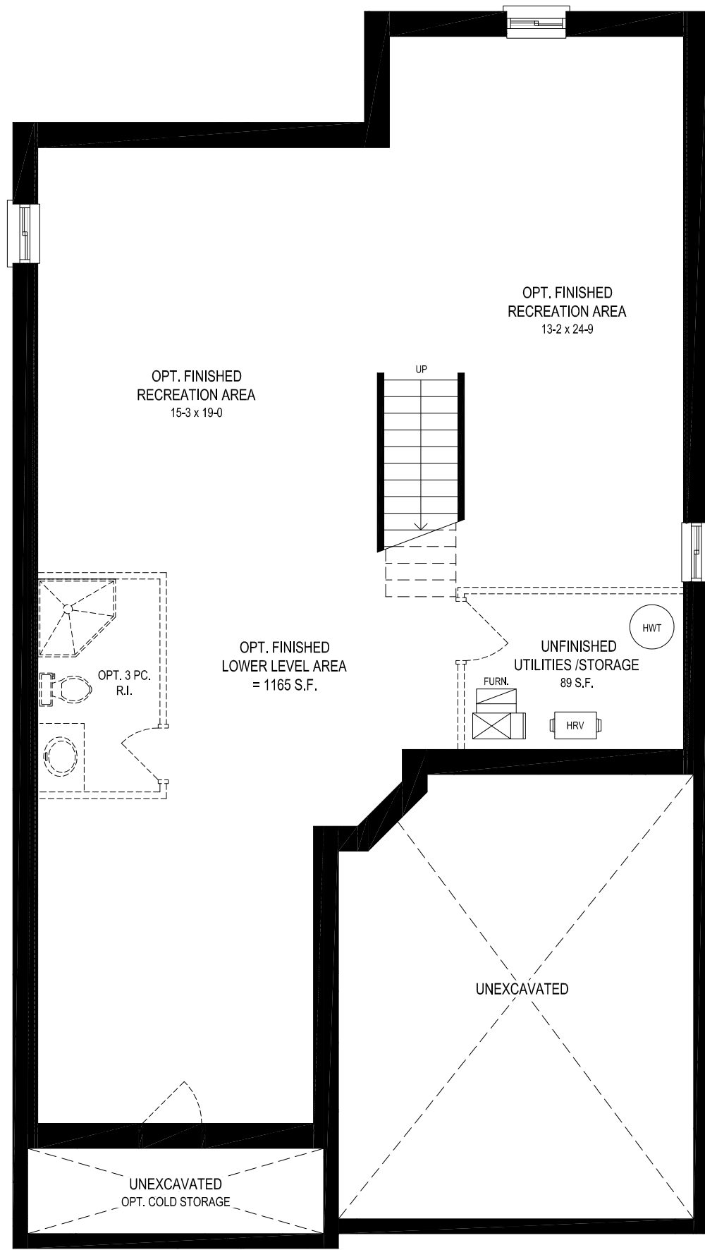
ALL ELEVATIONS - B1, LOWER LEVEL
