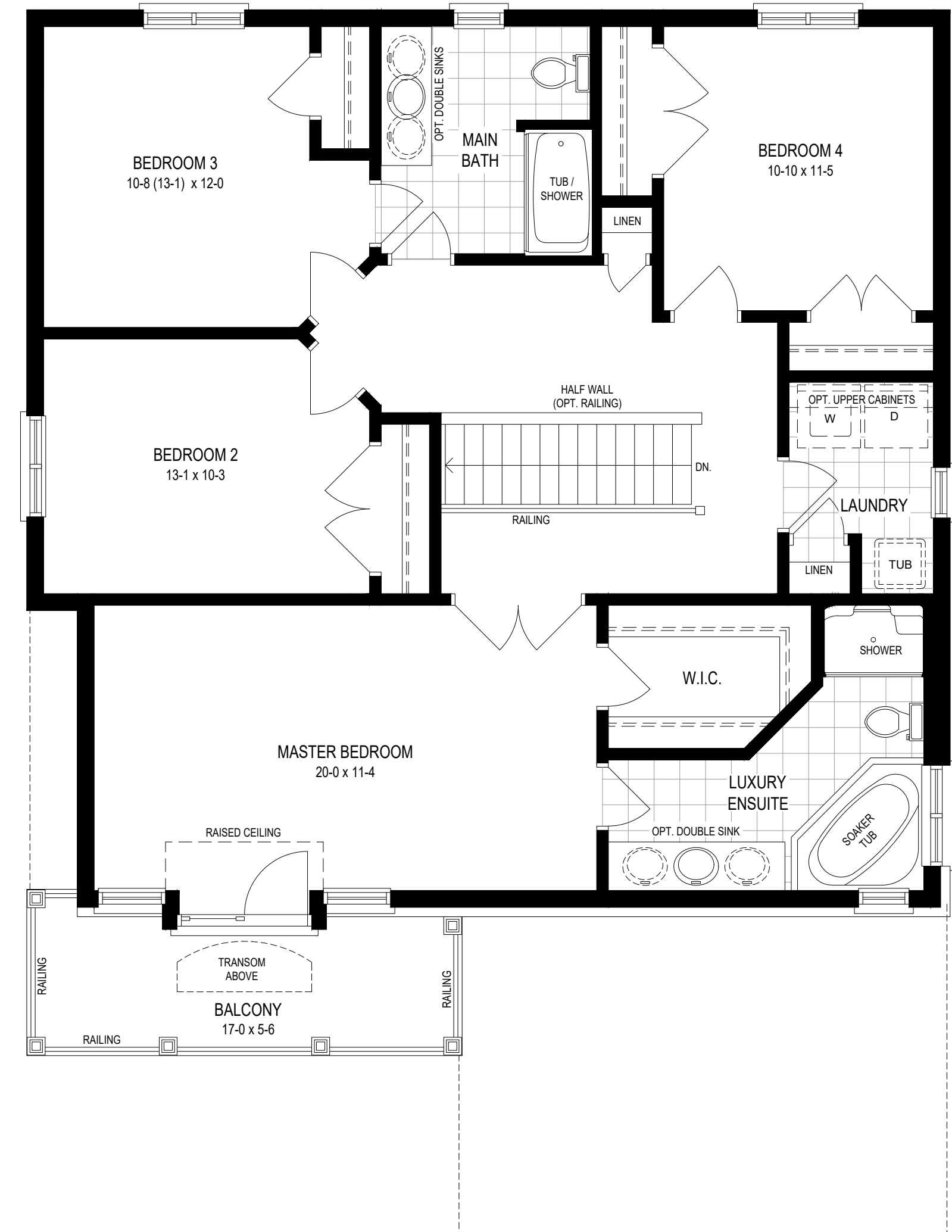
S1, SECOND FLOOR
