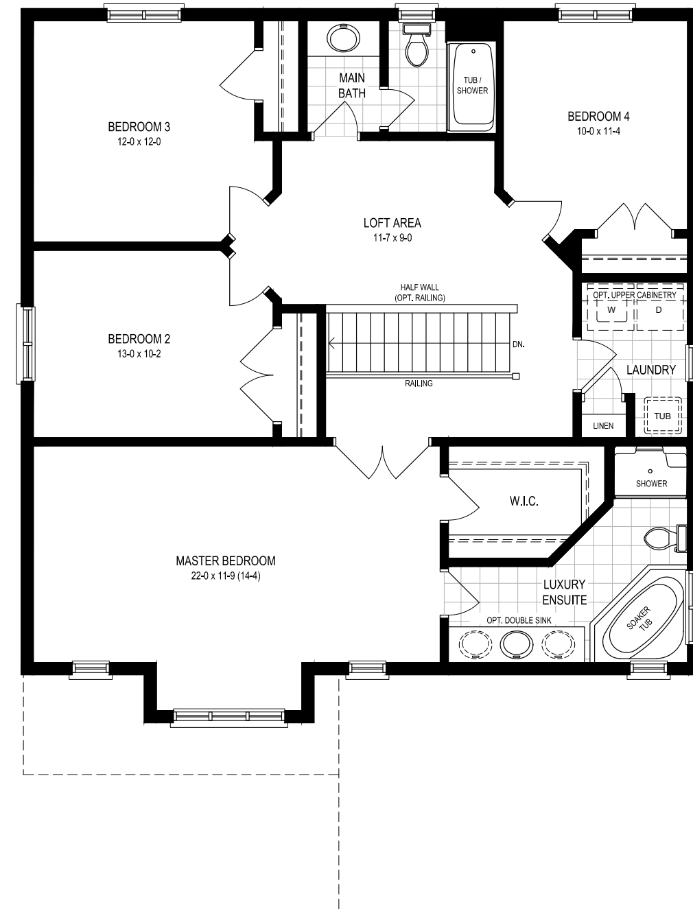
CHÂTEAU - S1, SECOND FLOOR
