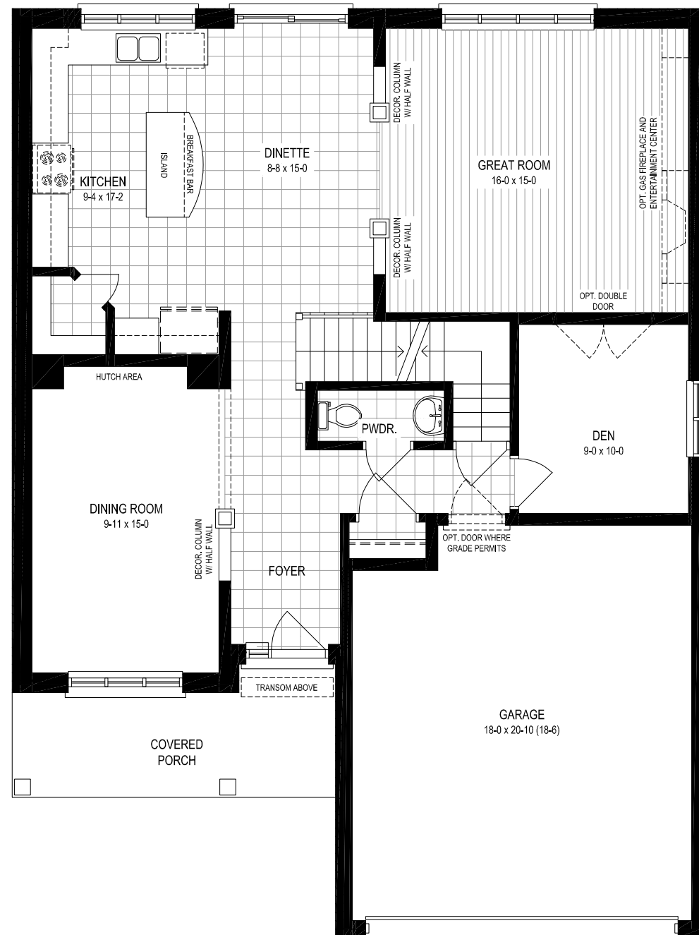
CHÂTEAU - M1, MAIN FLOOR
