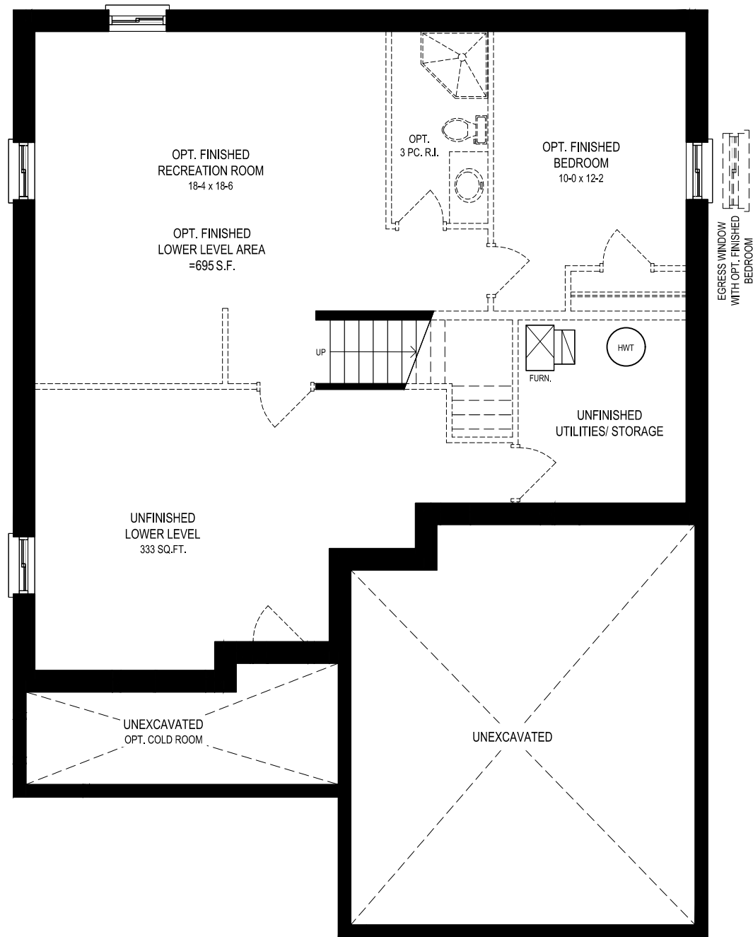
ALL ELEVATIONS - B1, LOWER LEVEL
