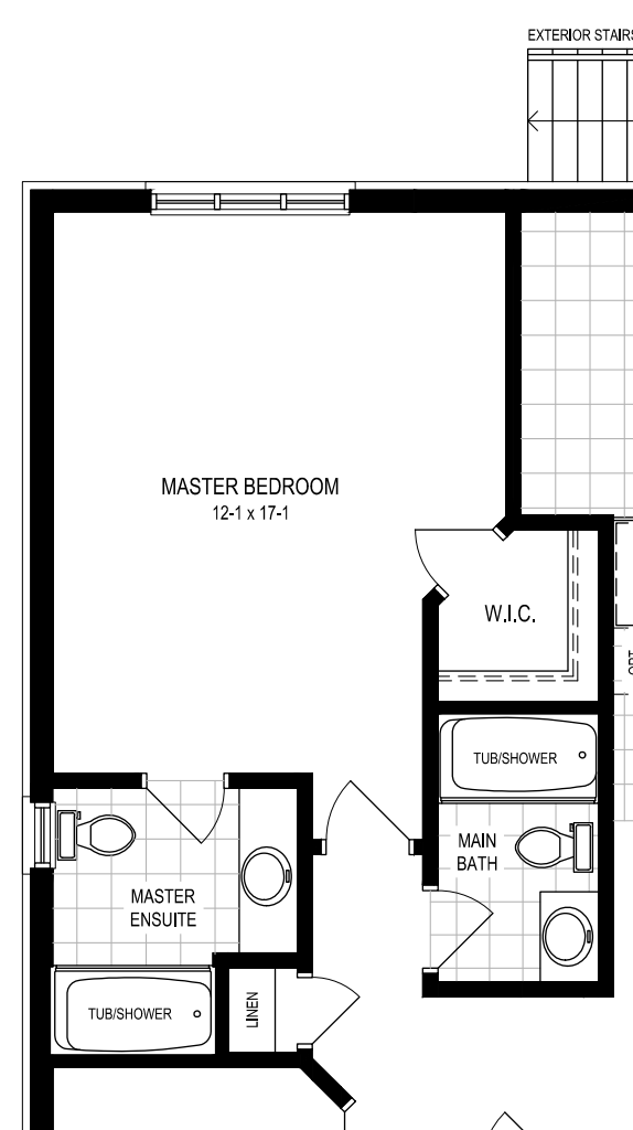
CHATEAU - M5, MAIN FLOOR
