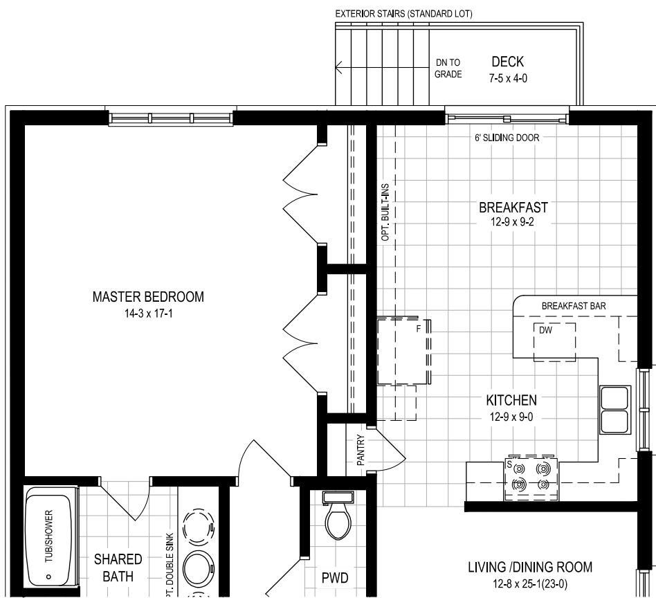
CHATEAU - B1, LOWER LEVEL
