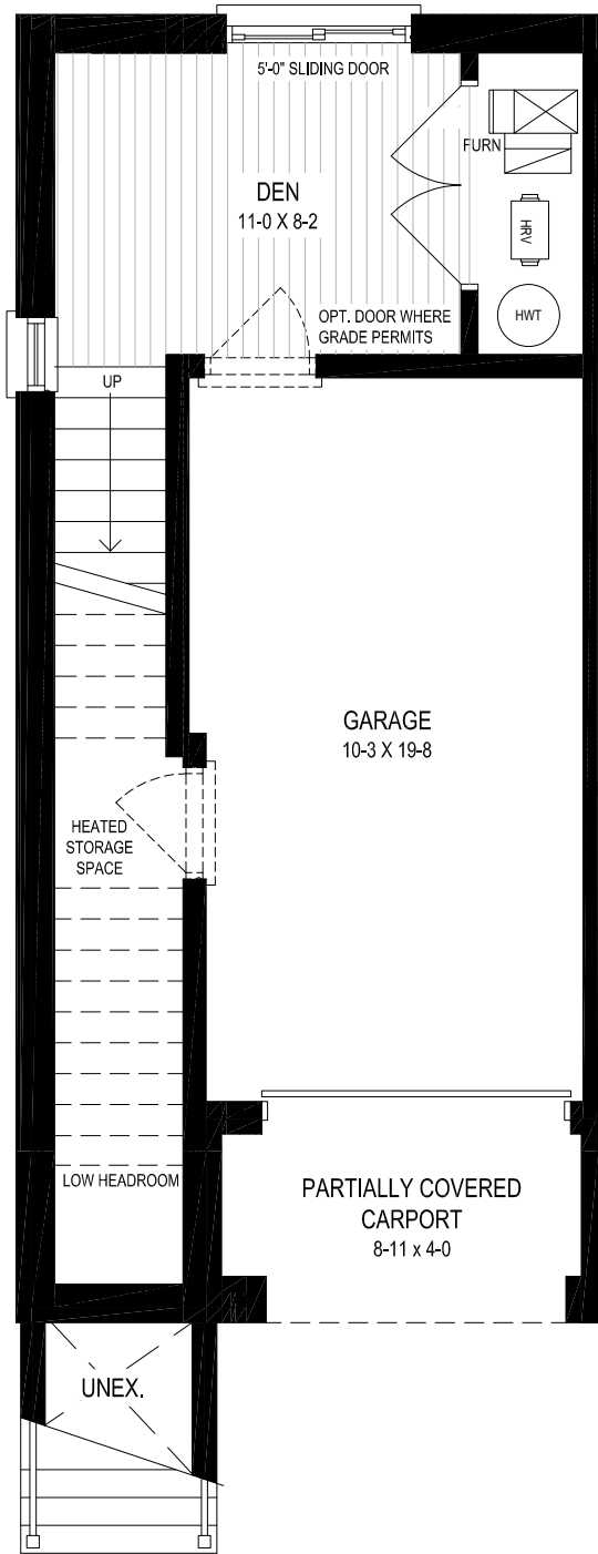
GROUND FLOOR
