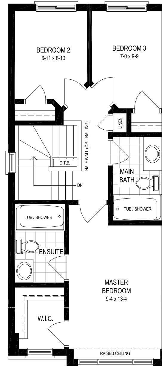
SECOND FLOOR
