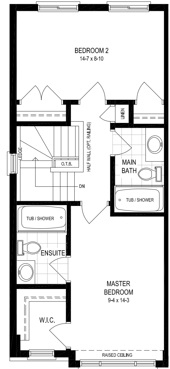
OPTIONAL SECOND FLOOR 2 BEDROOMS w ENSUITE
