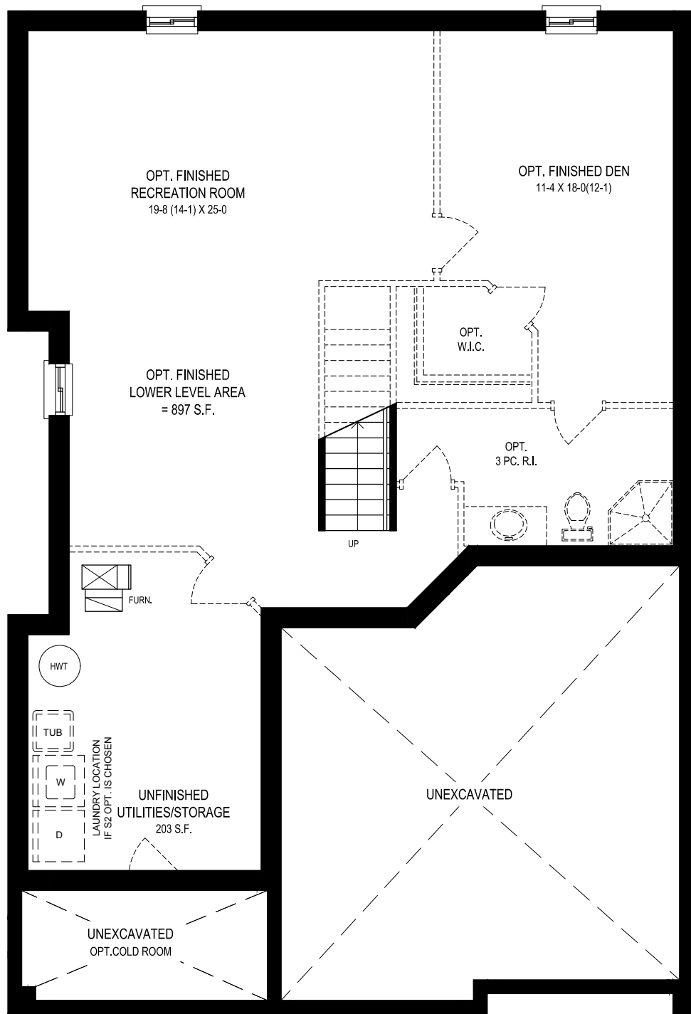
CHATEAU - B1, LOWER LEVEL
