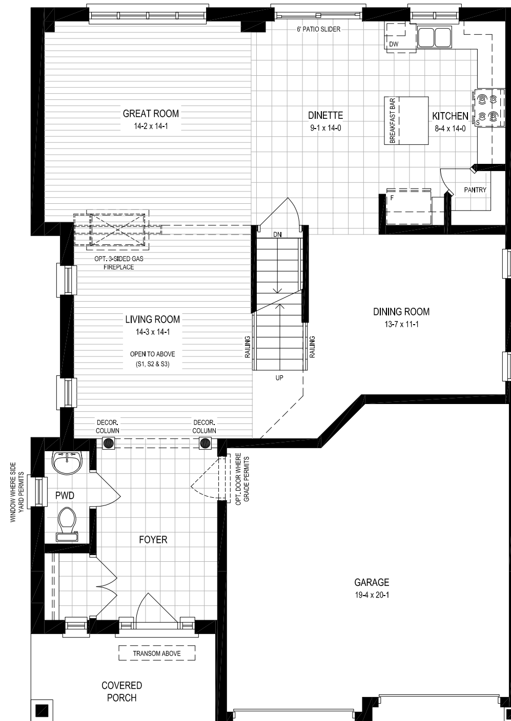
CHATEAU - M1, MAIN FLOOR
