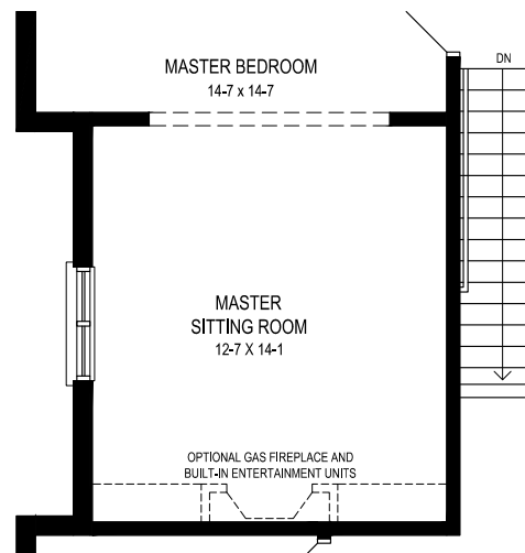
ALL ELEVATIONS - S4, SECOND FLOOR
