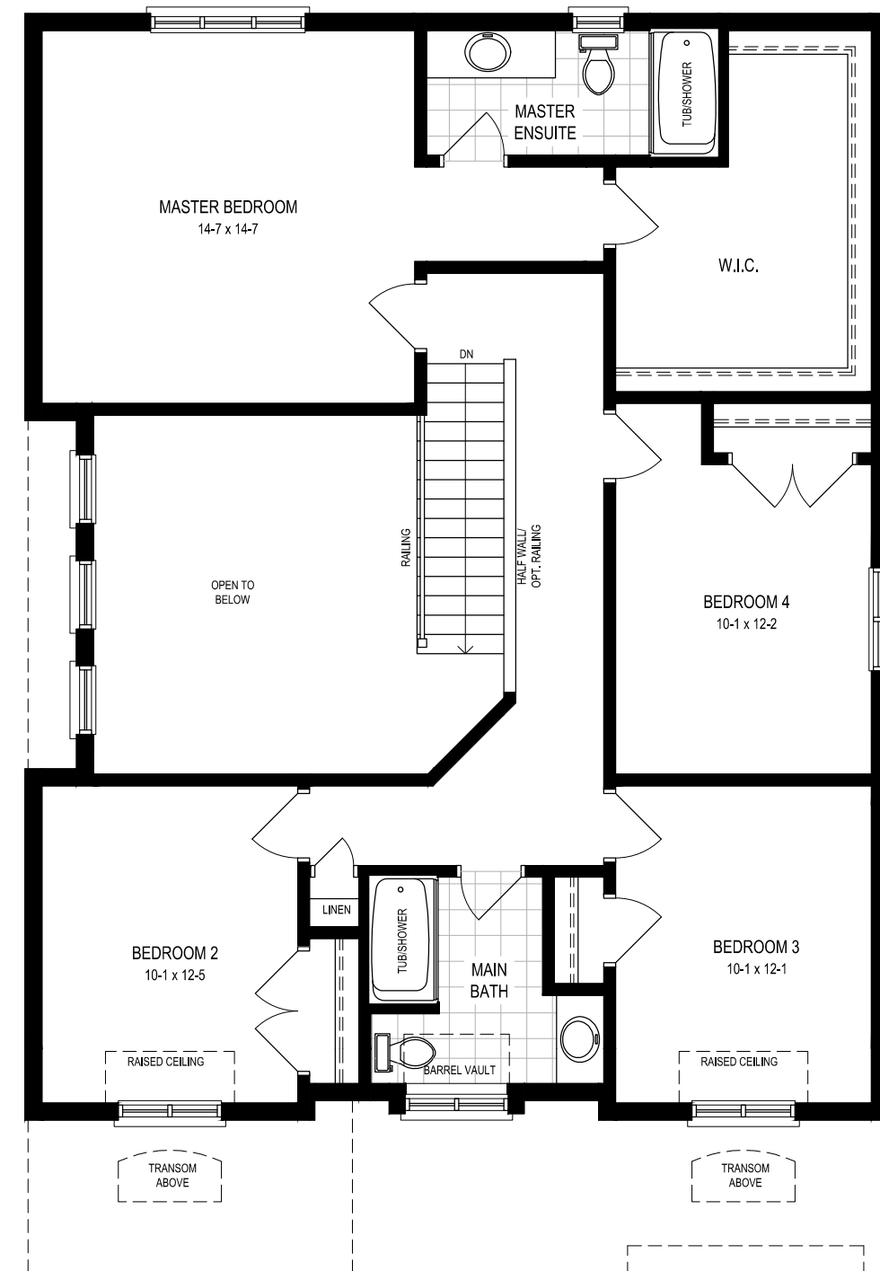
CHATEAU - S2, SECOND FLOOR
