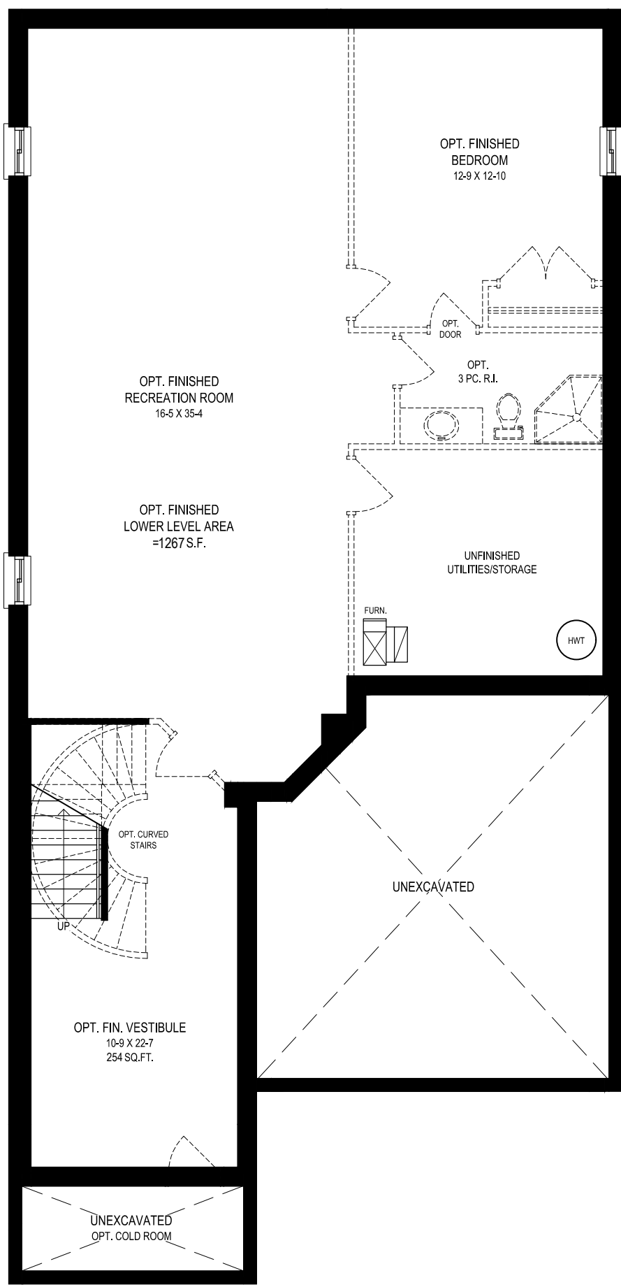
ALL ELEVATIONS - B1, LOWER LEVEL
