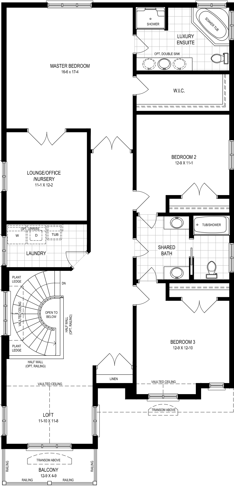
CHATEAU - S2, SECOND FLOOR
