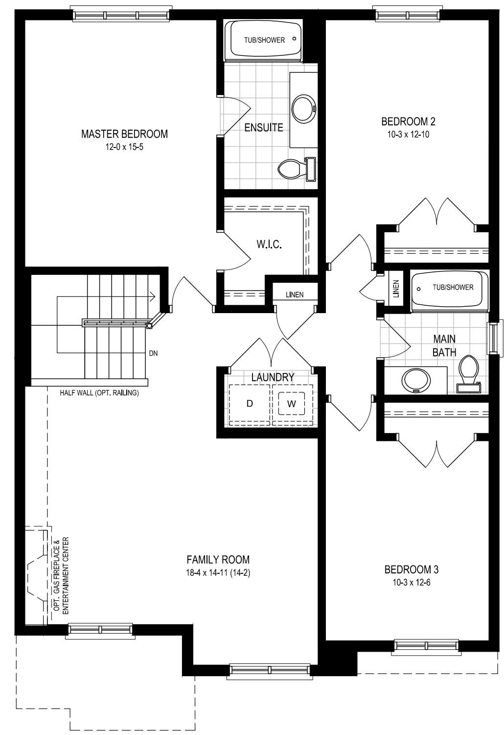
CHÂTEAU - S1, SECOND FLOOR
