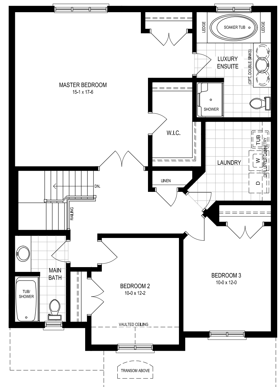
CHATEAU - S3, SECOND FLOOR
