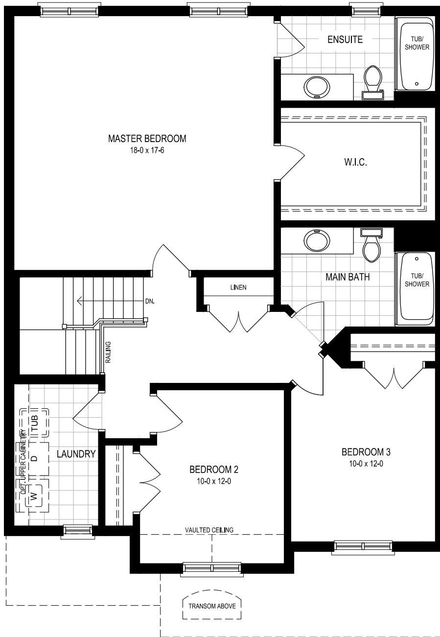
CHATEAU - S1, SECOND FLOOR
