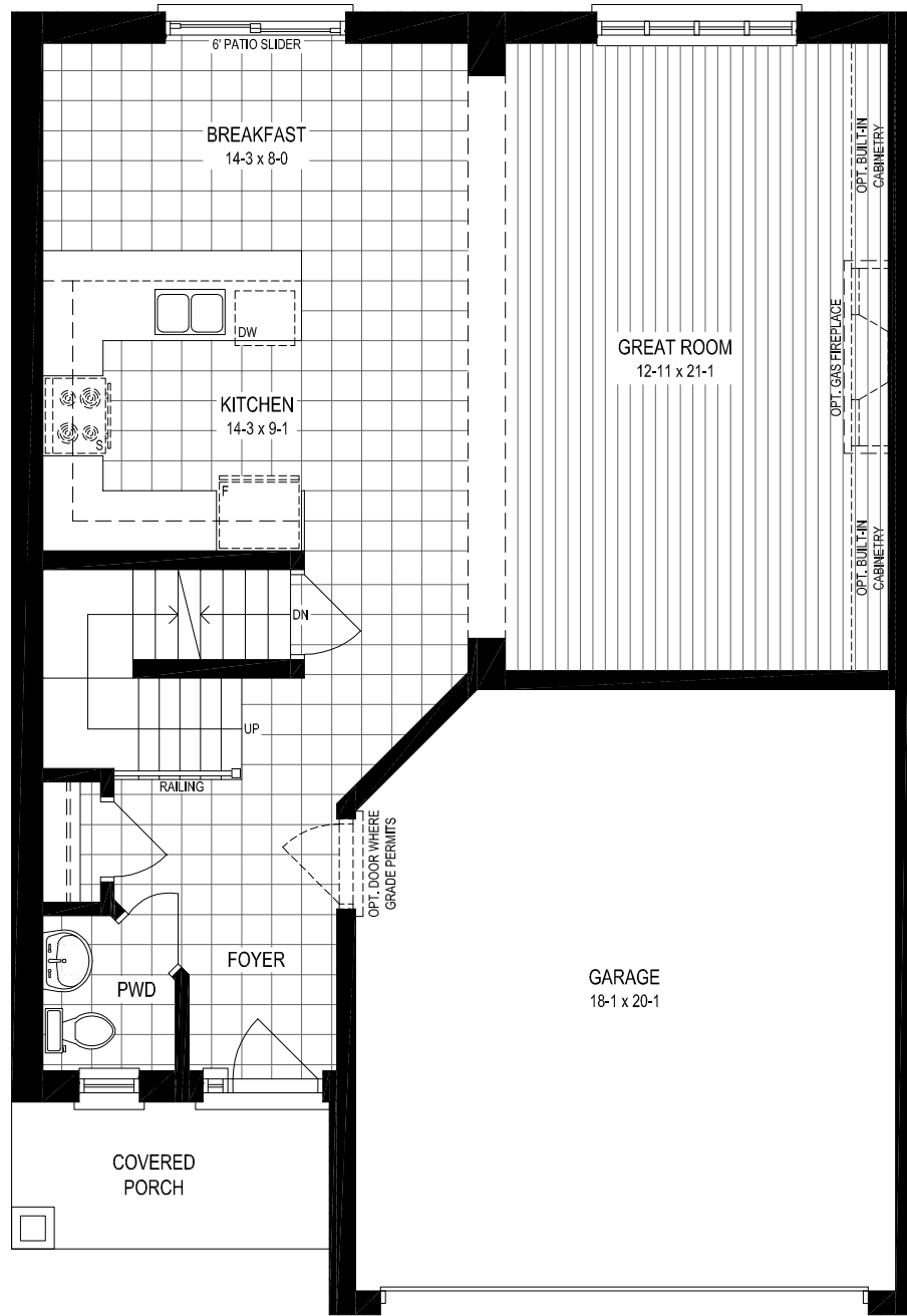
CHATEAU - M1, MAIN FLOOR
