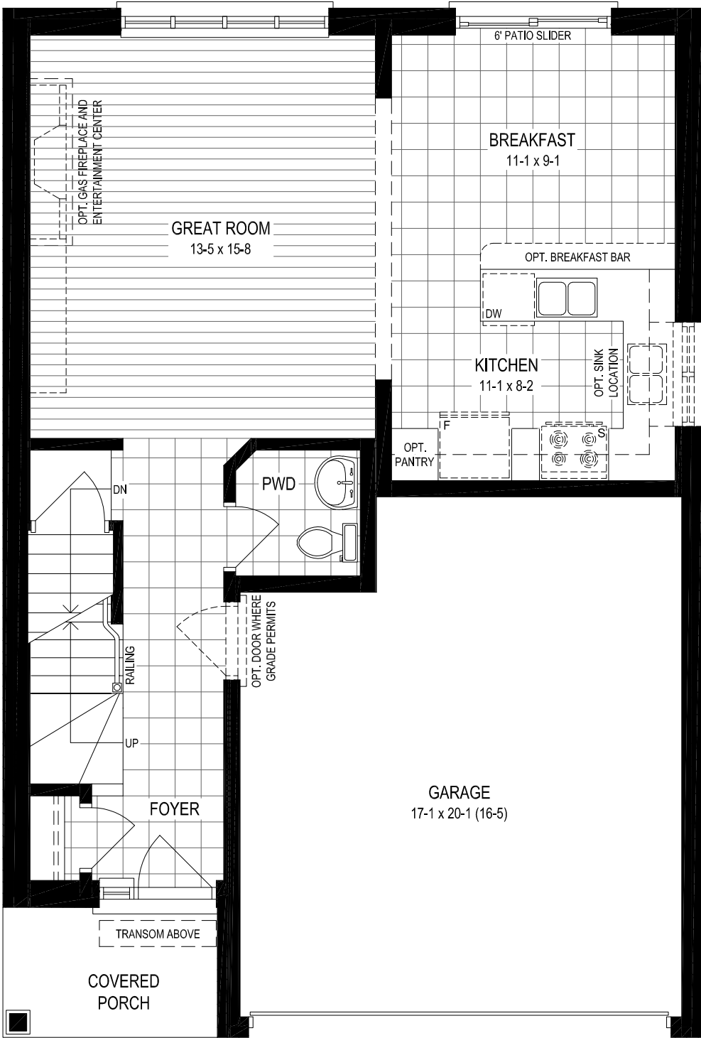
CHÂTEAU - M1, MAIN FLOOR
