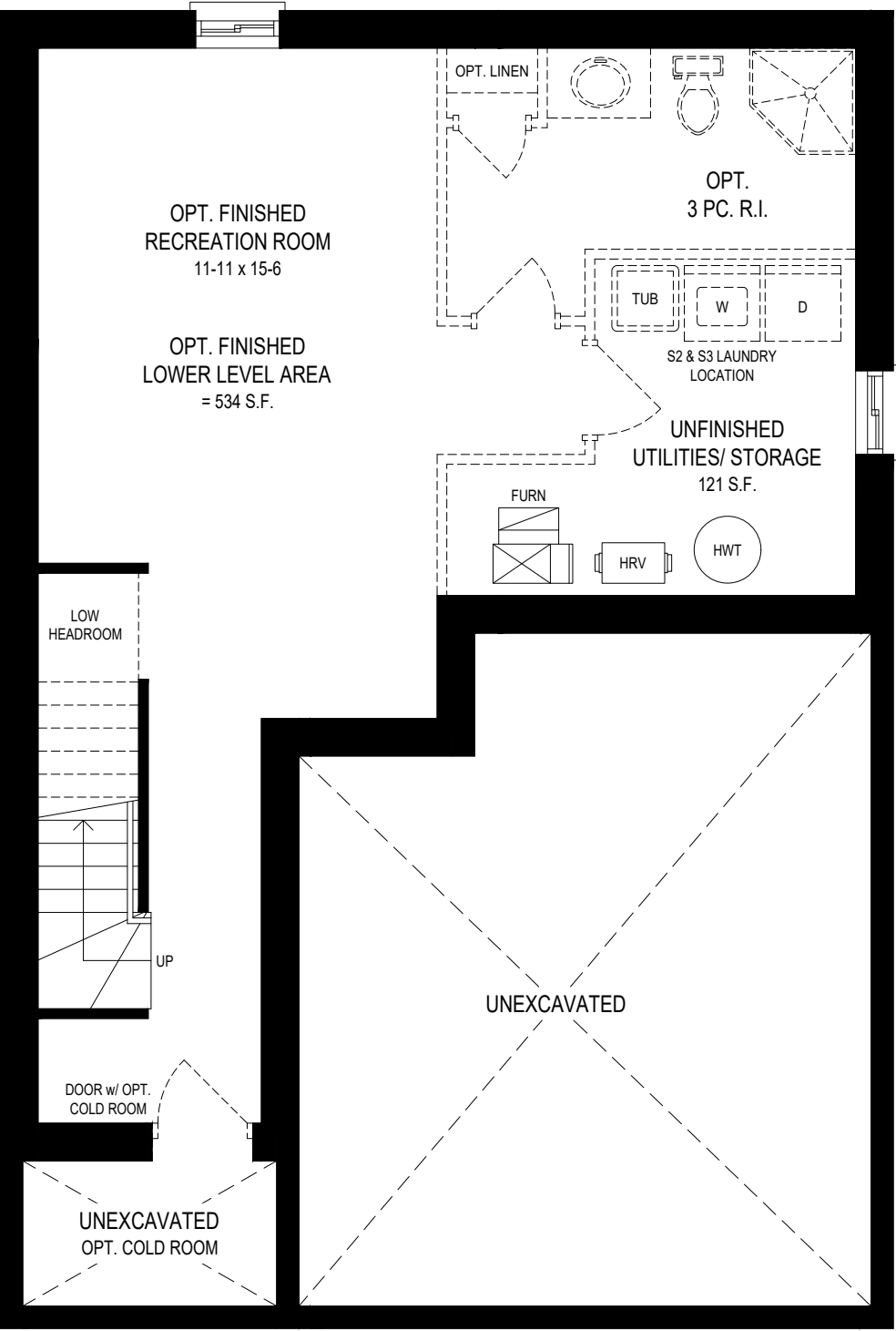
ALL ELEVATIONS - B1, LOWER LEVEL
