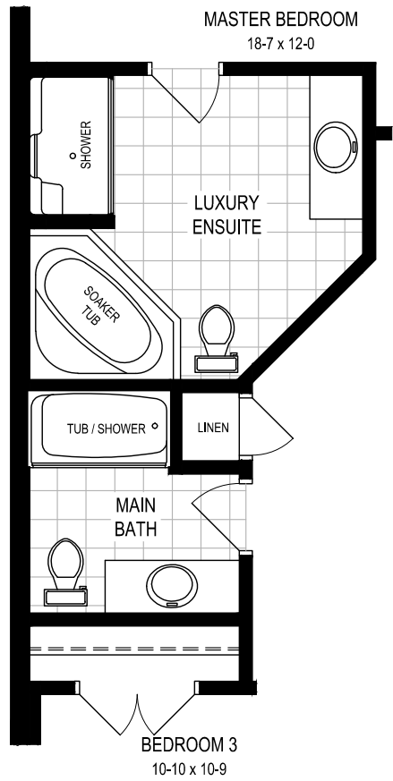
ALL ELEVATIONS - S2, SECOND FLOOR
