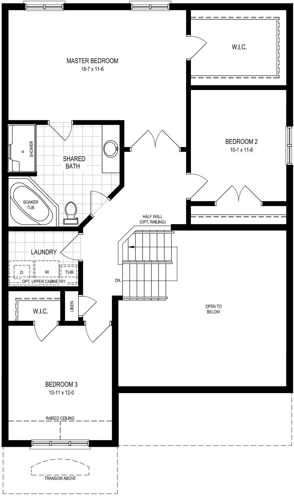
CHÂTEAU - S1, SECOND FLOOR
