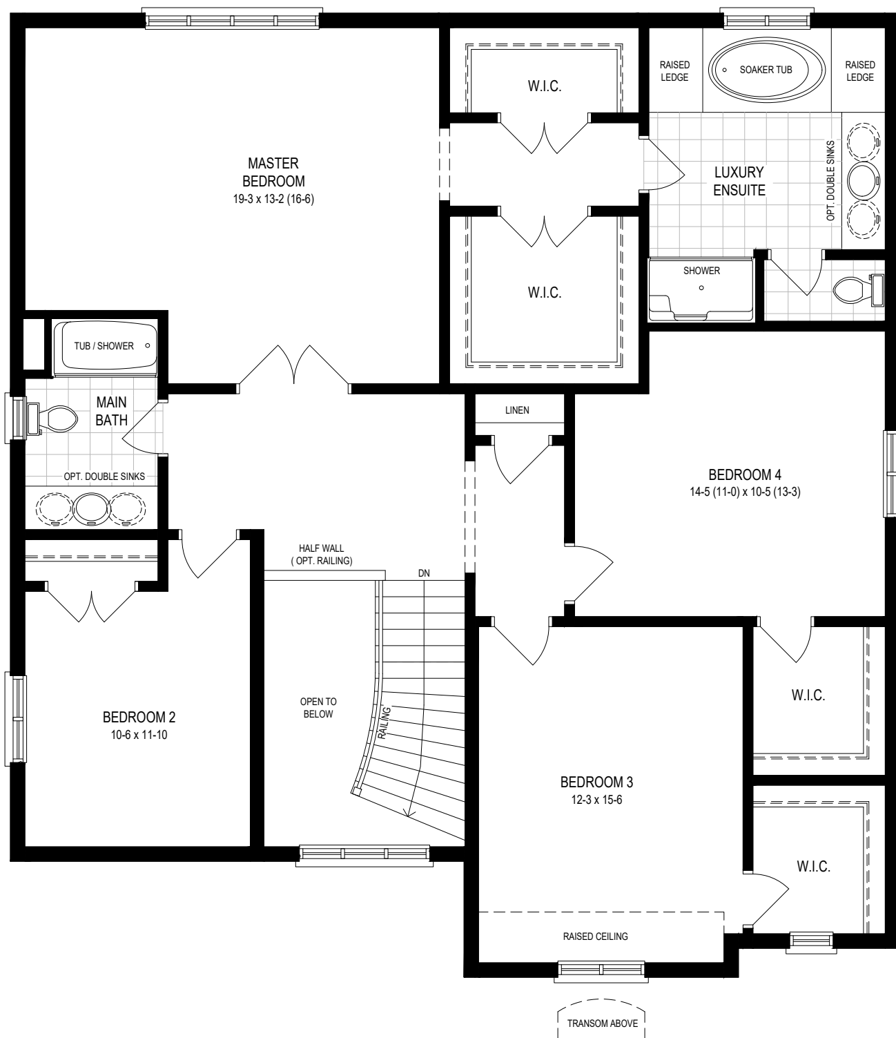
CHATEAU - S1, SECOND FLOOR
