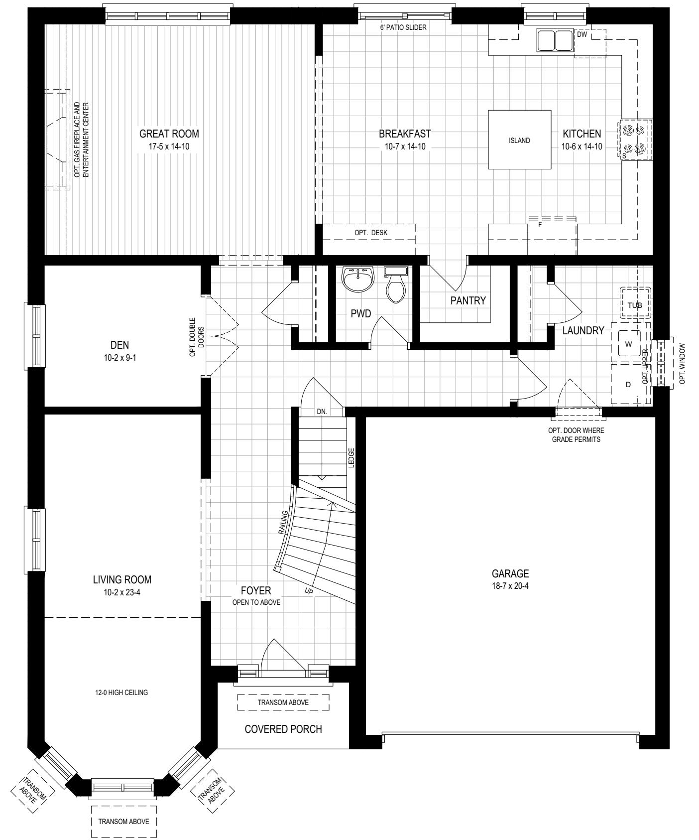
CHATEAU - M1, MAIN FLOOR
