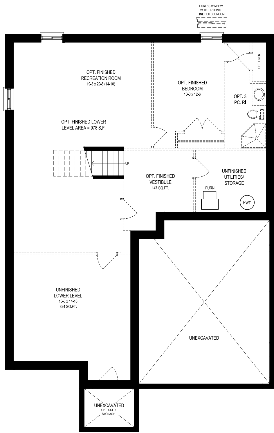
CHATEAU - B1, LOWER LEVEL
