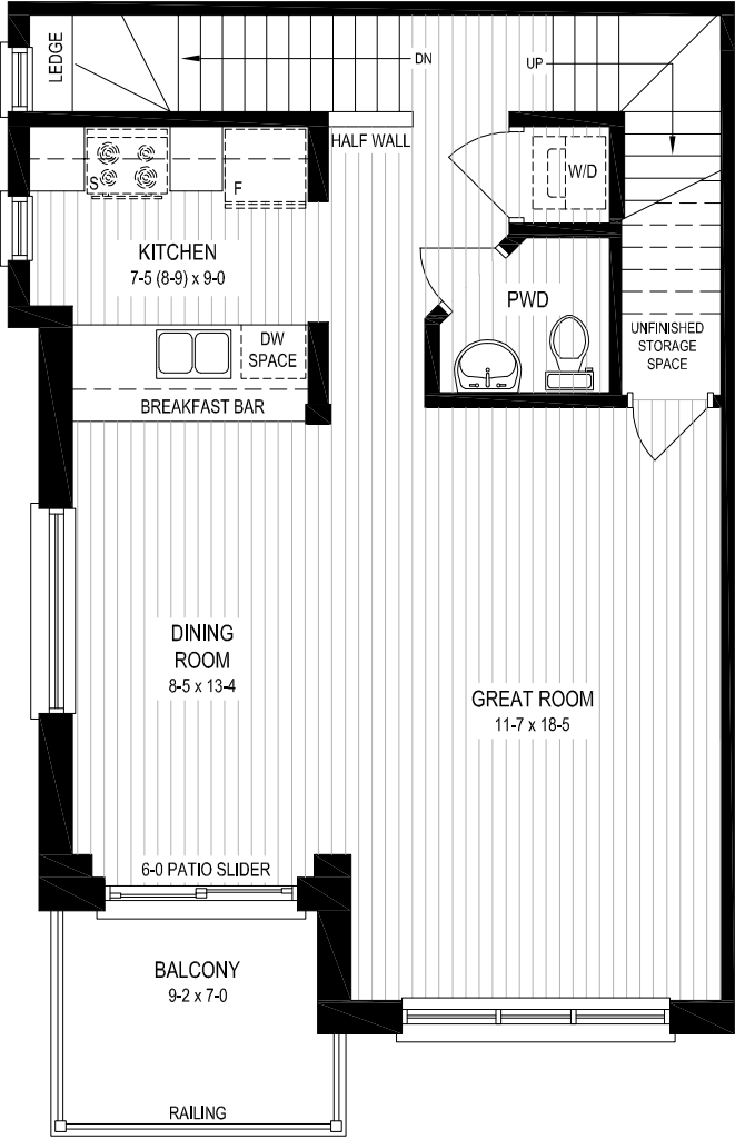
MAIN FLOOR
