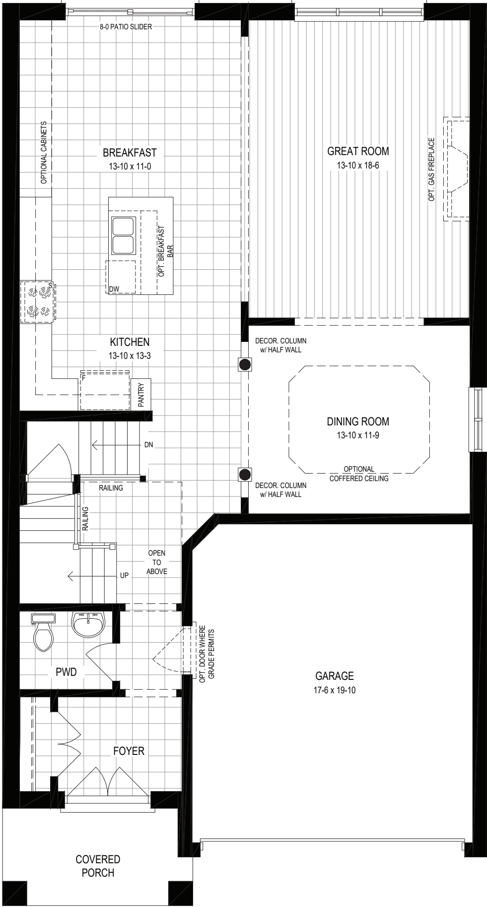
MAIN FLOOR
