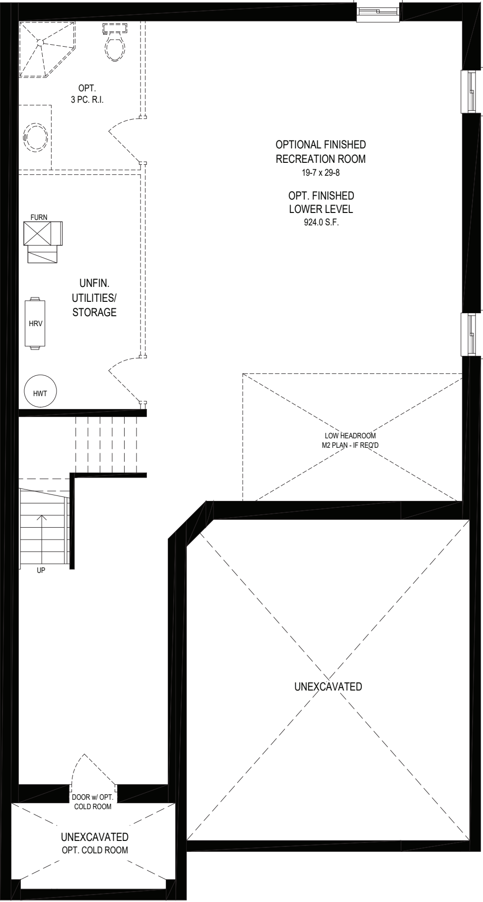
LOWER LEVEL
