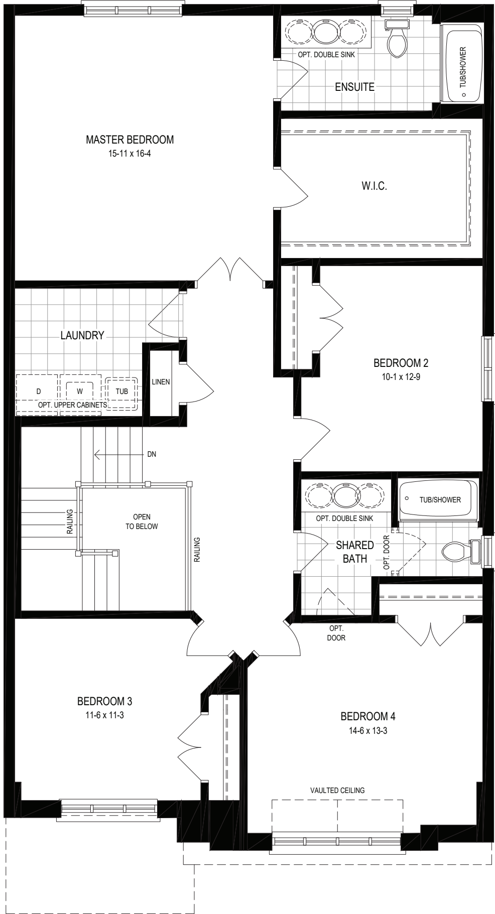
SECOND FLOOR
