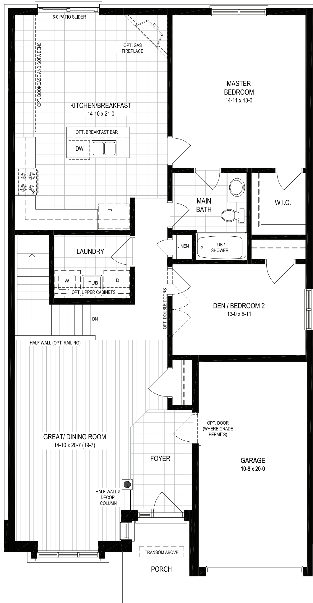
MAIN FLOOR
