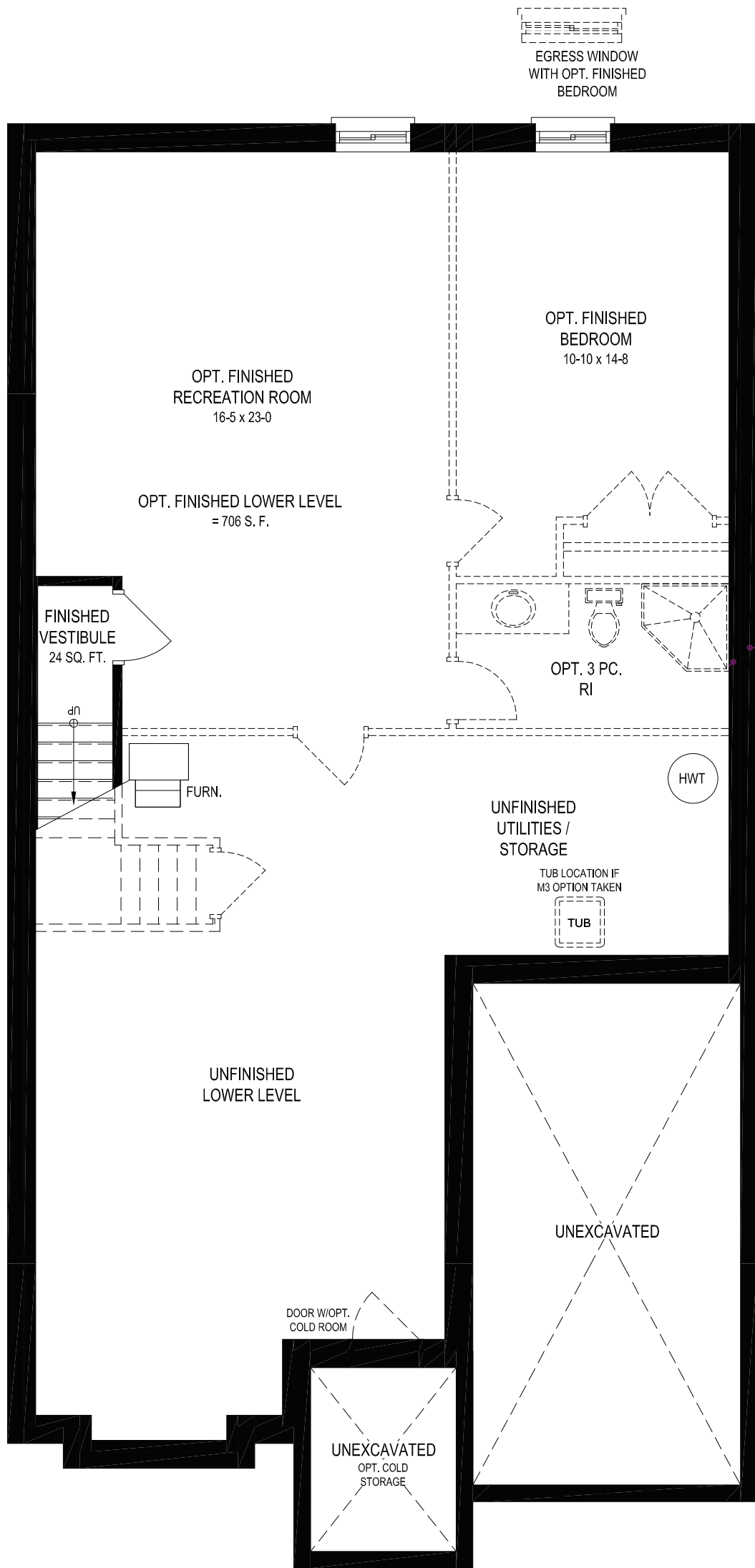
LOWER LEVEL
