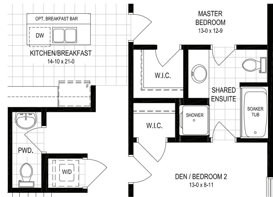
OPTIONAL MAIN FLOOR w/ SHARED ENSUITE & LAUNDRY CLOSET
