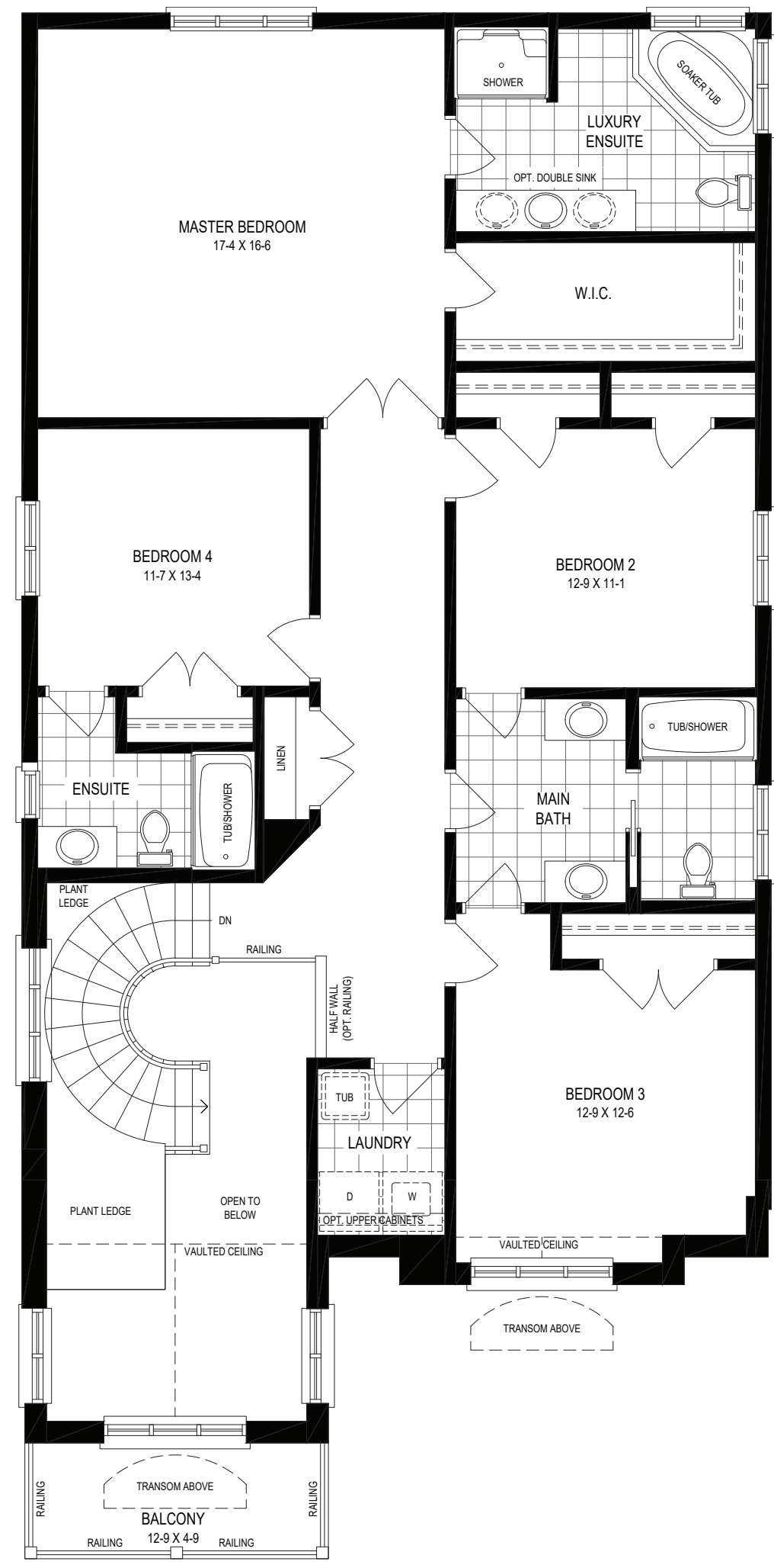
SECOND FLOOR
