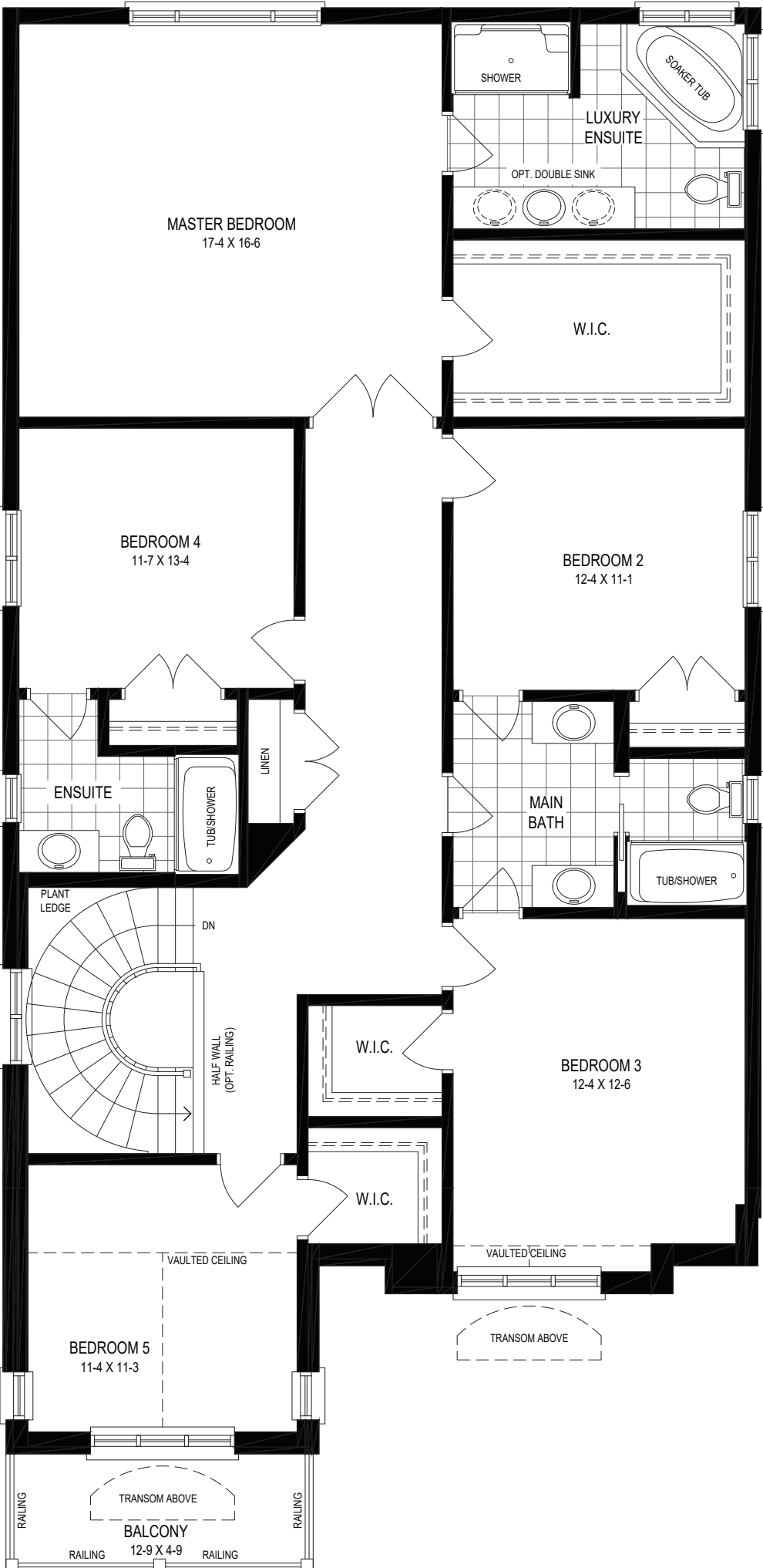
OPTIONAL SECOND FLOOR w/ 5 TH BEDROOM
