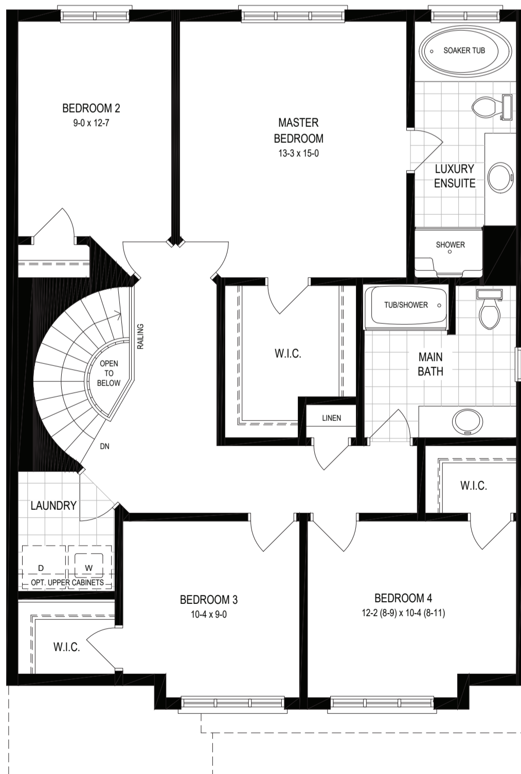
OPTIONAL SECOND FLOOR w/ LUXURY ENSUITE & ALTERNATE LAYOUT
