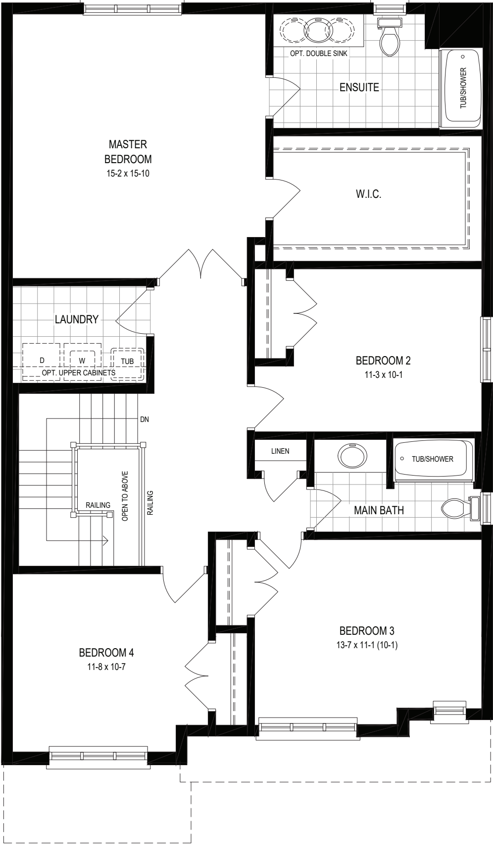
SECOND FLOOR
