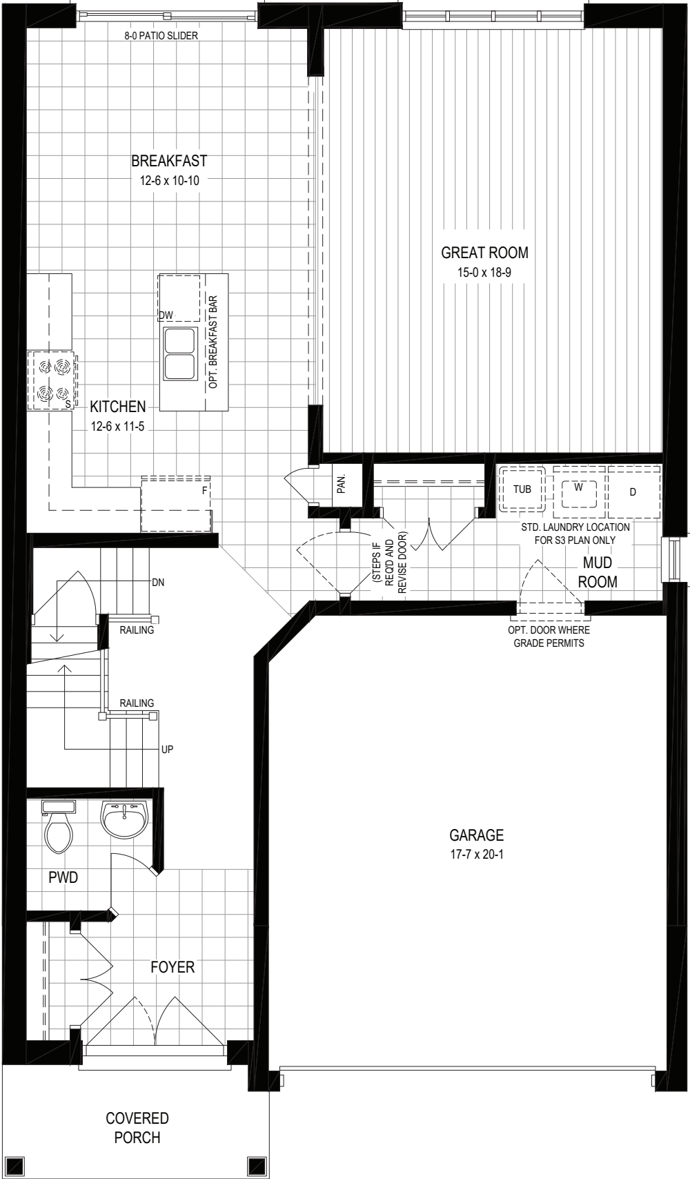
MAIN FLOOR
