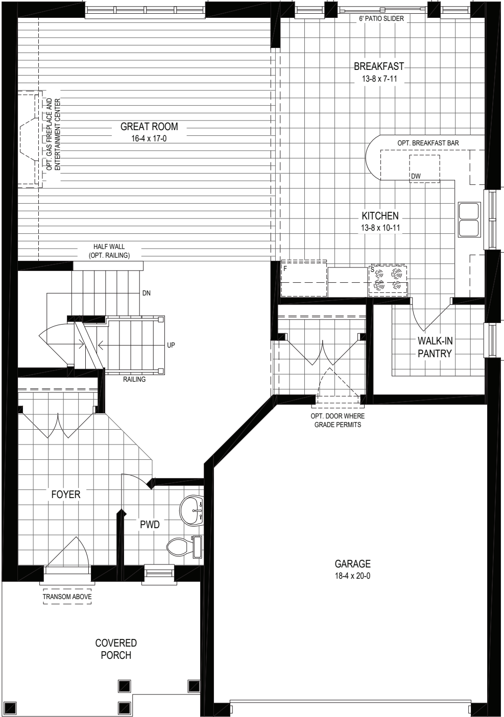
OPTIONAL MAIN FLOOR w/ WALK-IN PANTRY
