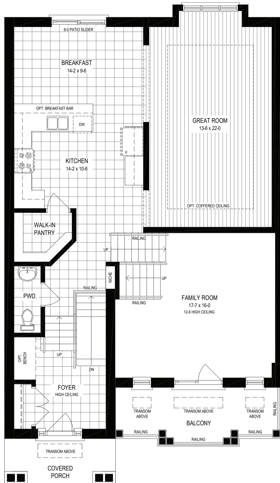
MAIN FLOOR
