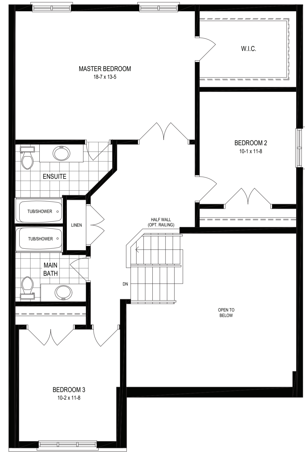
SECOND FLOOR
