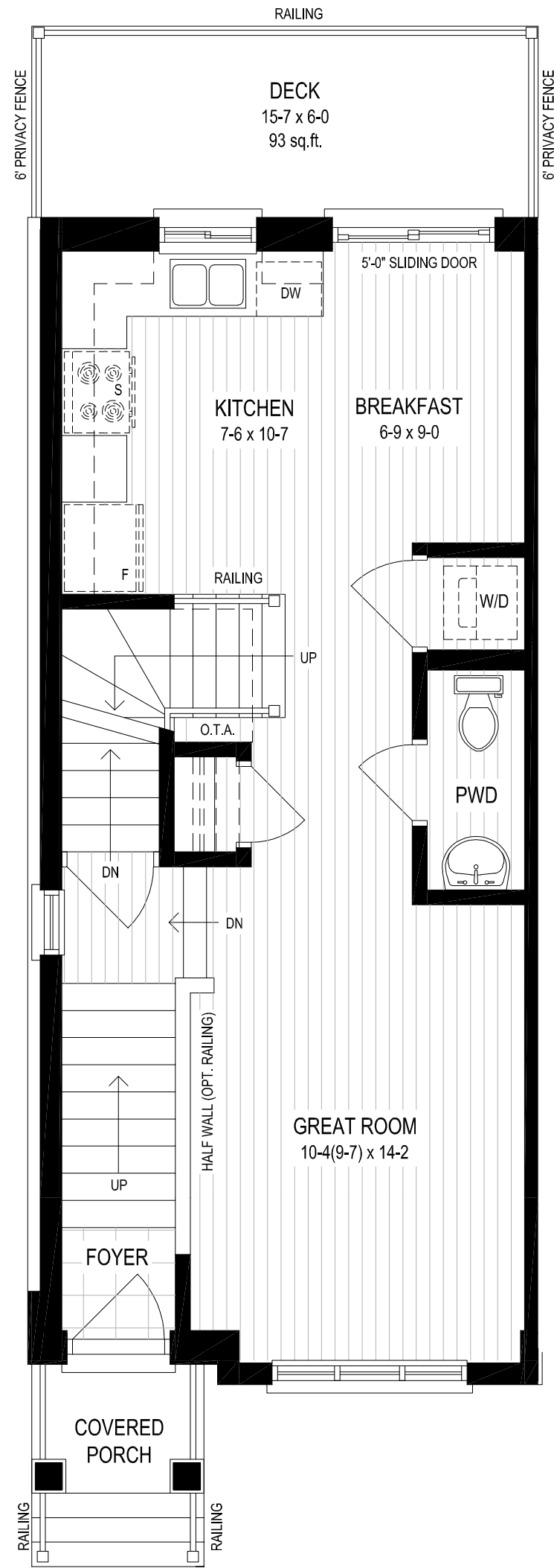
MAIN FLOOR
