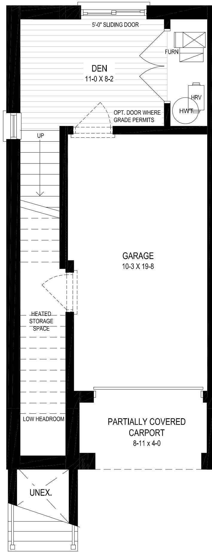
GROUND FLOOR
