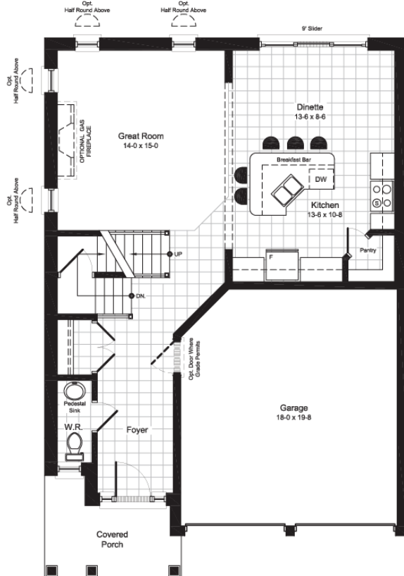
Standard Main Floor - M1 Elev. B
