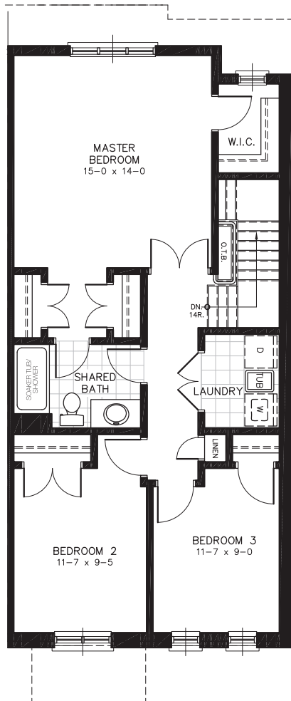
SECOND FLOOR – S1
