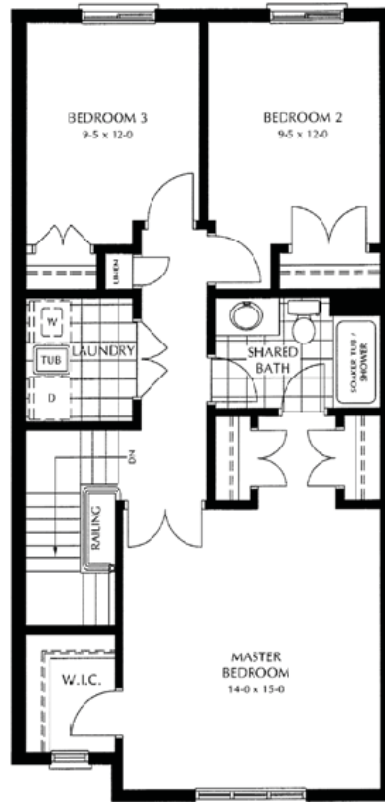
S1 - SECOND FLOOR PLAN
